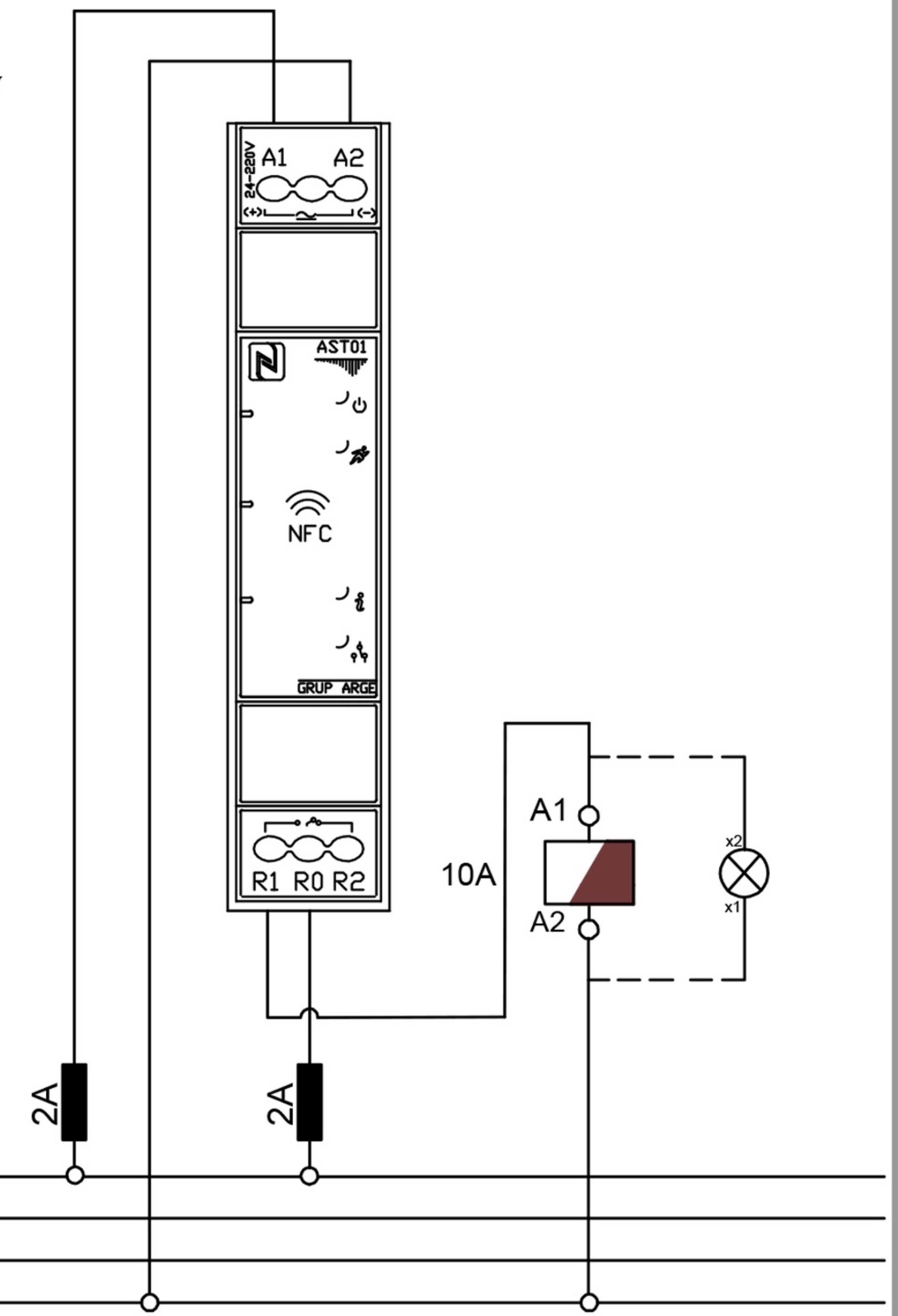
MONO-PHASE CONNECTION DIAGRAM
