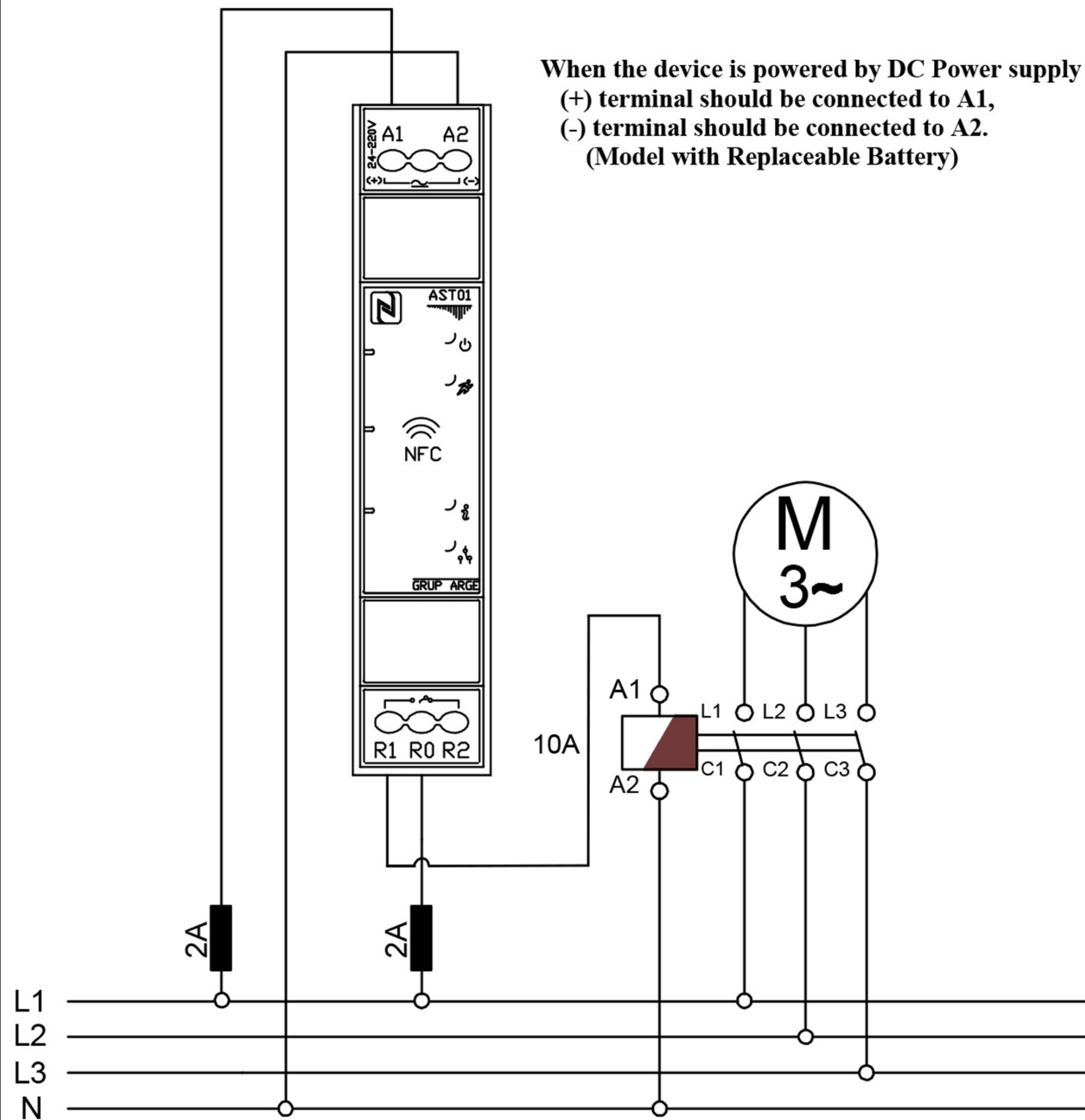
THREE-PHASE CONNECTION DIAGRAM
